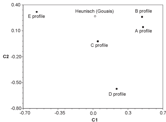
Fig. 2: Centroids of 5 'Wildbacher' genotypes and the 'Heunisch' ('Gouais') cultivar obtained with genetic similarity values.
