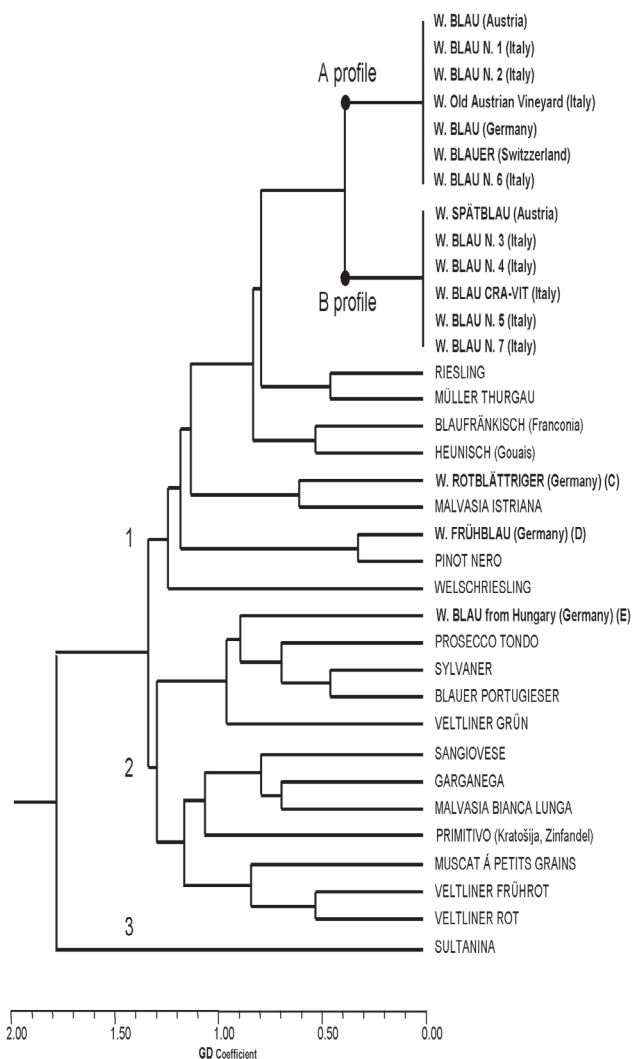
Fig. 1: Dendrogram of 16 'Wildbacher' accessions plus 19 outgroup varieties and Austrian cultivars (cophenetic correlation value: 0.8485), obtained with genetic dissimilarity indices.
