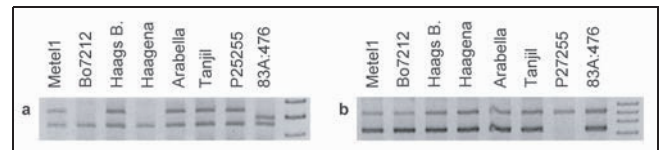
Fig. 4. Screening of SSR markers VIII003F04 obtained from Medicago truncatula (a) and Lotus japonicus (b).
