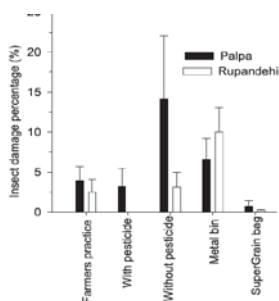
Fig. 7 Insect damage after 6 months in wheat seed versus storage method, Nepal (Devkota et. al., 2017)
