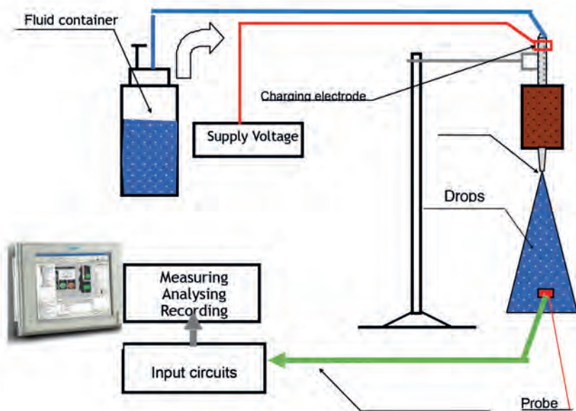
Fig. 1. Laboratory stand.
