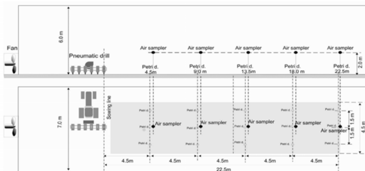
Fig. 1. The layout of CRA-ING testing area for checking pneumatic drills.
