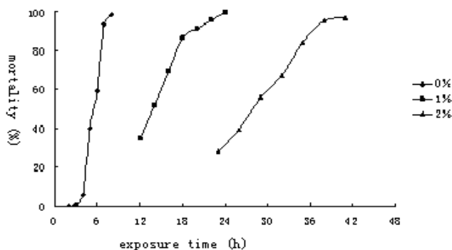
Figure 1 The mortality curve of L. bostrychophila adults in three different low oxygen concentrations.
