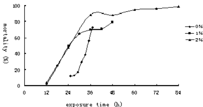
Figure 7 The mortality curves of S. zeamais at three different treatments of low oxygen.
