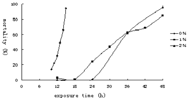
Figure 4 The mortality curves of T. castaneum (Yiyang) at three different treatment of low oxygen.
