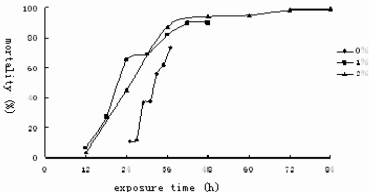
Figure 6 The mortality curves of S. oryzae at three different treatment of low oxygen.
