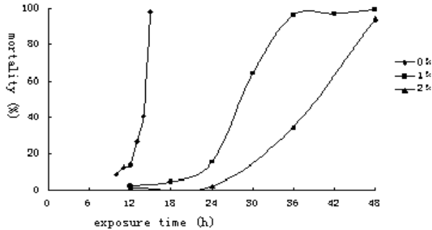
Figure 3 The mortality curves of T. confusum at three different treatment of low oxygen.
