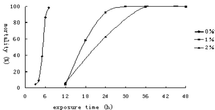
Figure 2 The mortality curves of O. surinamensis in three different low oxygen concentrations.
