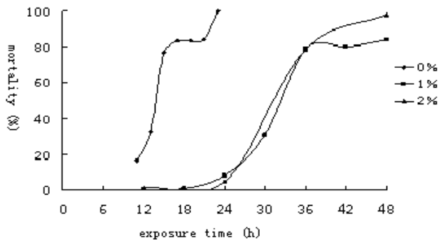
Figure 5 The mortality curves of T. castaneum (Zhongshan) at three different treatment of low oxygen.
