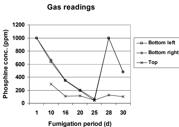
Figure 1 Phosphine concentrations in the silo under fumigation at Clifton for validation of the fumigation protocol of 360 ppm for 30 days.
