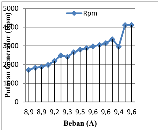
Gambar 6. Grafik Putaran Generator (Rpm) Terhadap Beban (A)
