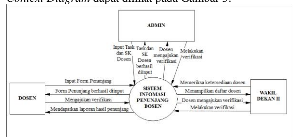
Gambar 5. Context Diagram
