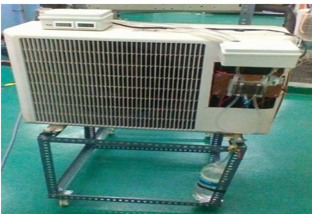
Figure 6: Overall experiment layout
