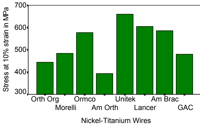
Diagram 2 Stress at 10% strain for nickel-titanium wires
