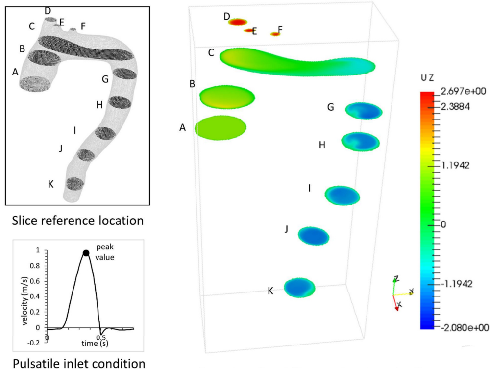
Fig. 6. Velocity contour at several slice locations during the time of the peak flow. The left bottom subfigure is pulsatile flow imposed at the inlet
