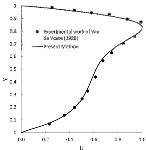
Fig. 1. Flow solver validation. The flow solver agrees closely with experimental results measured in the center plane of the tube at the end of the curved section
