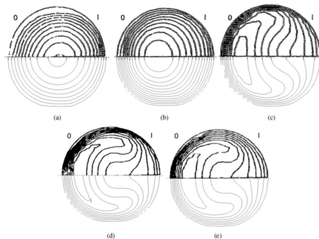
Fig. 2. Velocity contour maps; a) 0 degree, b) 22.5 degree, c) 45 degree, d) 67.5 degree and e) 90 degree, (I: inner curve, O: outer curve). The results presented in the upper half of the figure were derived by Van de Vosse et al. , [19]. Our numerical results are given in the bottom half
