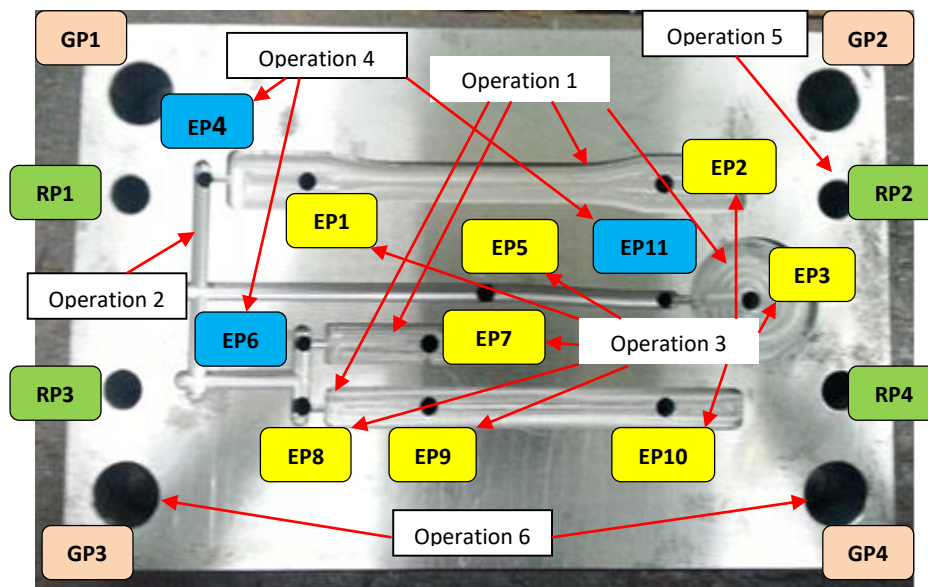
Figure 5 The core plate of the family mould
