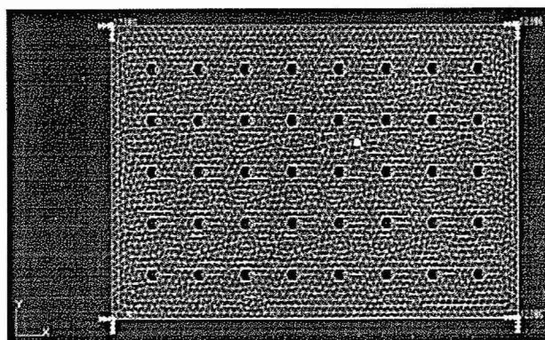
Figure 2. FE model of a perforated panel with 40 holes and 10 mm hole diameter.
