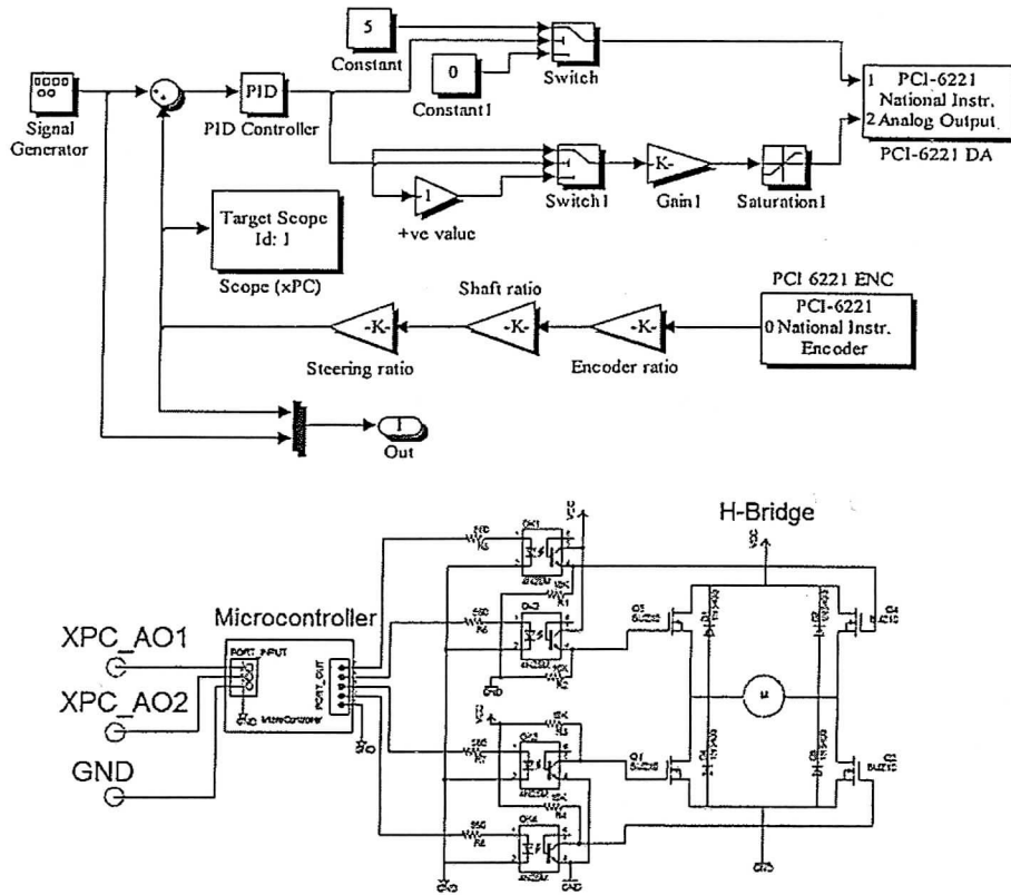
Figure 2 a) position controller develop for HIL via XPC target. b) DC motor circuit
