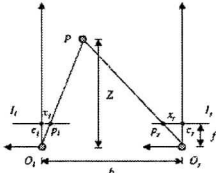
Figure 2. Basic principle of stereo vision
