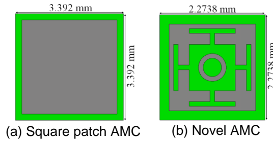
Figure 5. A unit cell AMC at 28 GHz
