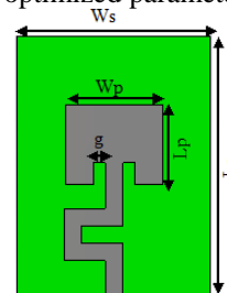
Figure 3: Configuration of insert feed line antenna
