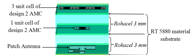
Figure 12: Configuration of multilayer patch antenna with design 2 AMC
