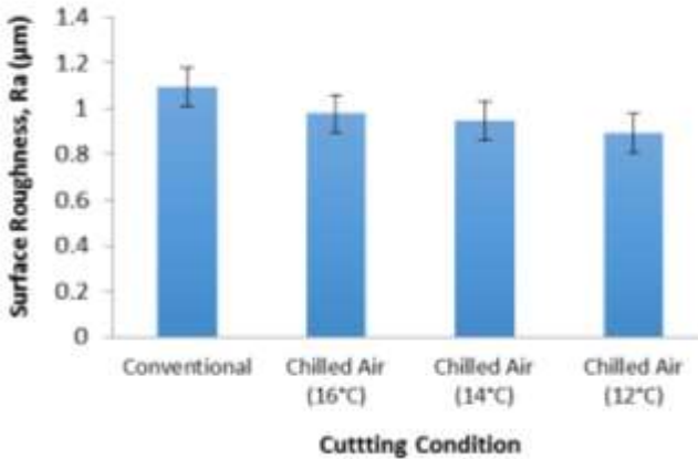
Figure 2: Surface roughness for all cutting conditions
