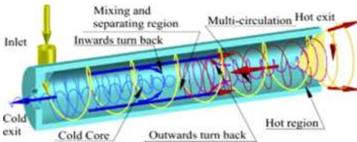
Figure 1: The structure of the flow inside a counter flow vortex tube [7]
