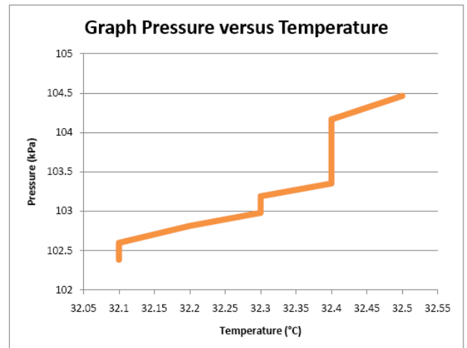
Figure 7 Relationship between pressure and temperature
