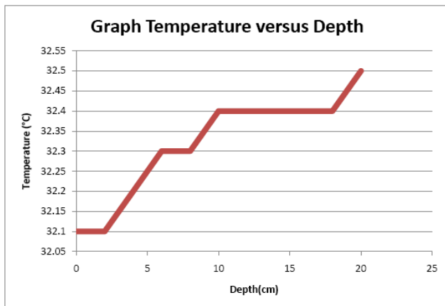
Figure 6 Relationship between temperature and depth
