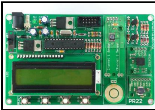
Figure 3(b) PCB circuit board (PR22)
