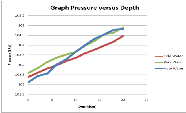
Figure 8 Graph pressure versus depth for all testing method
