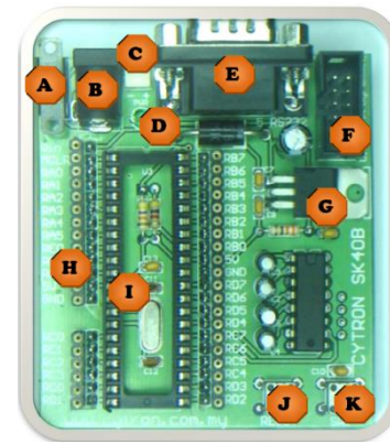
Figure 2 Board layout [2]
