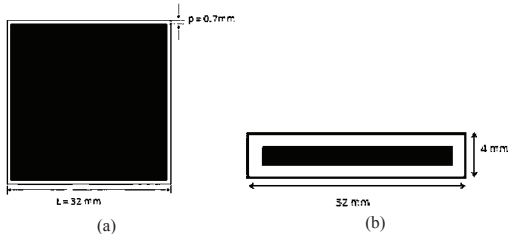
Figure 3: Schematic and dimensions of two AMCs (a) Square AMC structure (b) Rectangular AMC structure [8]
