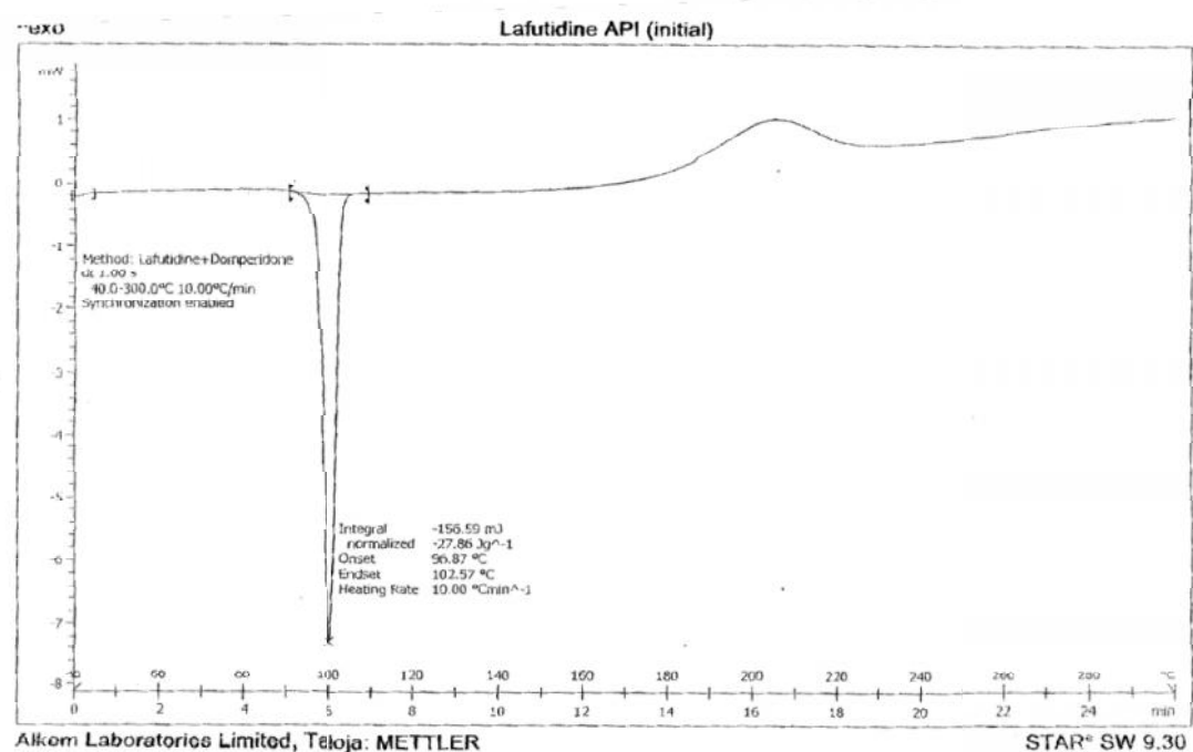
Figure 6: DSC thermograph of Lafutidine (Initial)
