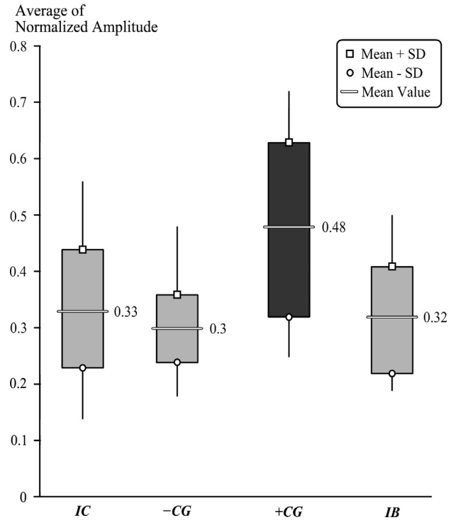
Fig. 13. Statistical distribution of the averaged normalized amplitude for IC, –CG, +CG and IB groups.
