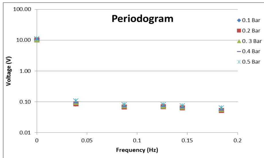
Fig. 5: Comparison Periodogram data of 30W PEMFC with various hydrogen pressures.
