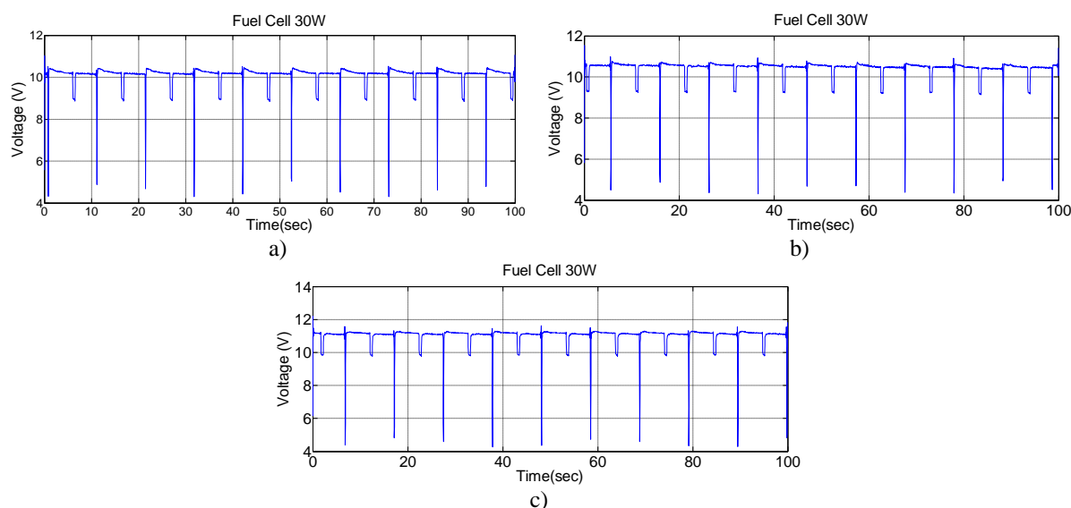
Fig. 2: Performance voltage (V) of 30W PEMFC with different of hydrogen ( H_2 ) pressure at anode side: a) 0.1 bar H_2 pressure b) 0.3 bar H_2 pressure c) 0.5 bar H_2 pressure.
