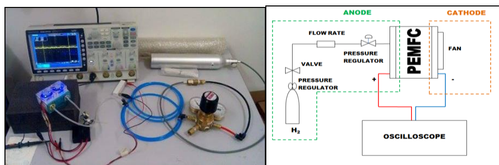
Fig. 1: Schematic diagram of experimental setup with oscilloscope and pressure regulator.
