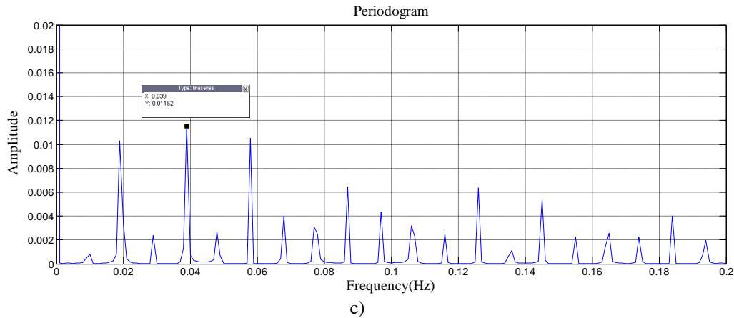
Fig. 4: Periodogram of 30W PEMFC with different of hydrogen ( H_2 ) pressure at anode side: a) 0.1 bar H_2 pressure b) 0.3 bar H_2 pressure c) 0.5 bar H_2 pressure
