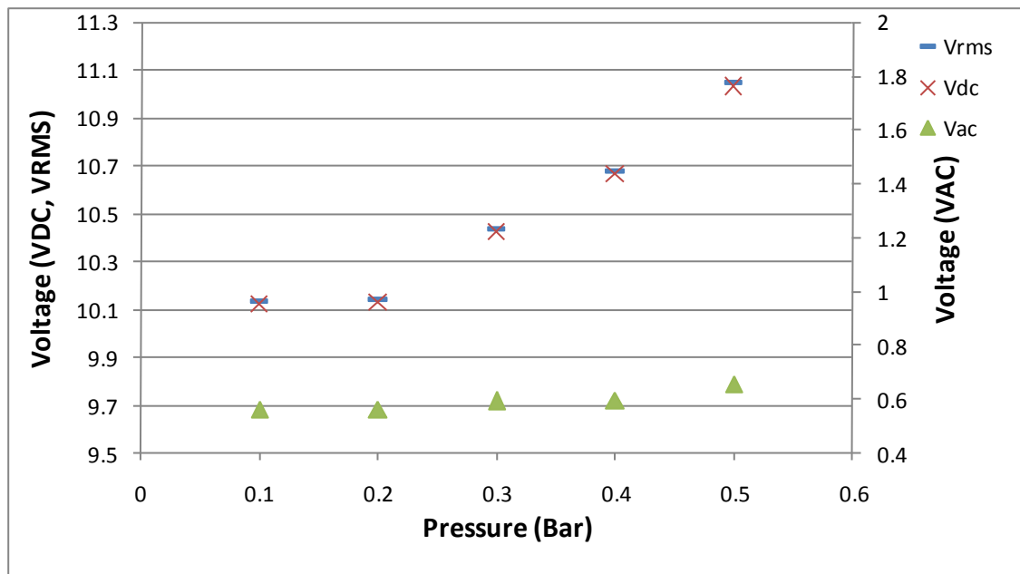
Fig. 6: Periodogram data of V_{DC} , V_{RMS} , and V_{AC} at various pressures.
