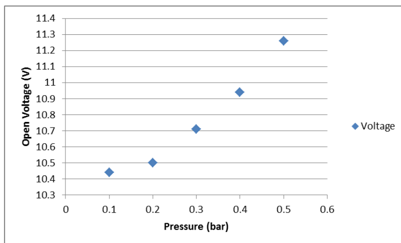
Fig. 3: Effect of pressure towards the PEMFC voltage at open voltage condition.
