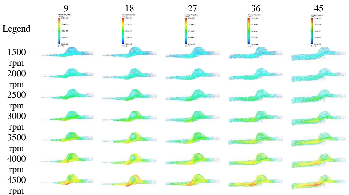
Figure 6. Flow Viewed from Plane B
