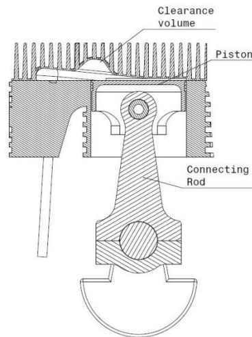
Figure 1: Clearance volume of the in-cylinder engine
