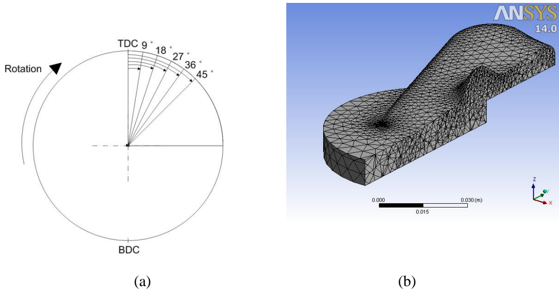
Figure 3. (a) Complete cycle; (b) Cut-view of the clearance volume of engine
