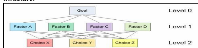
Figure 1 : Illustrative a simple AHP Model
