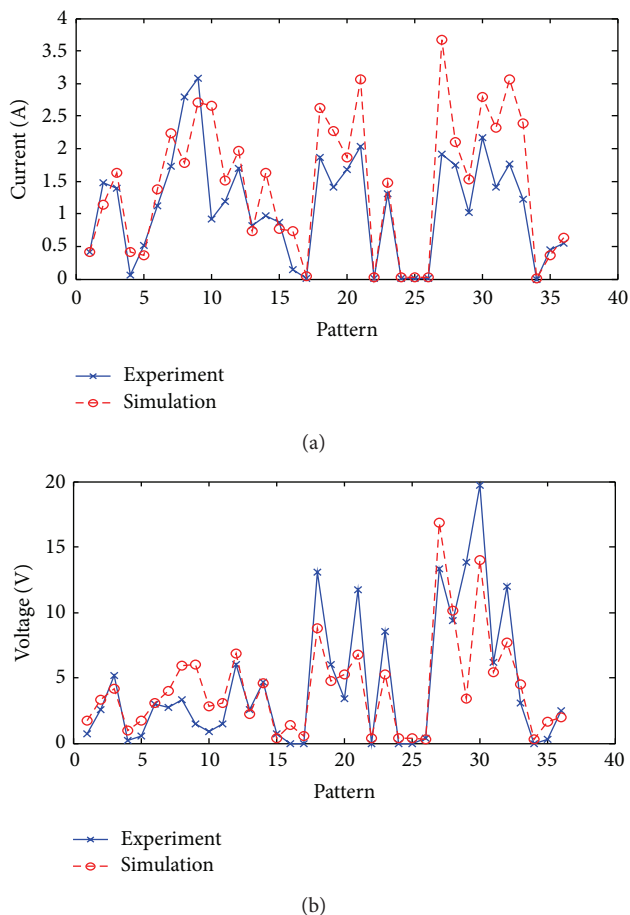
FIGURE 6: Comparisons of ANN predictions (test data) and experimental results for current and voltage in 5 hidden neurons.
