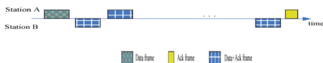
Fig. 1. Piggyback mechanism
