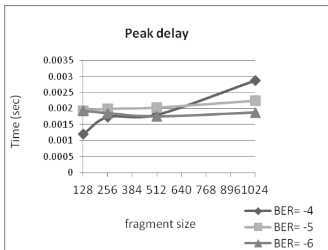
Fig. 8. Peak delay compared with fragmentation size
