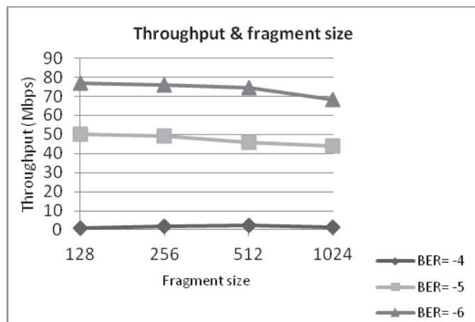
Fig. 7. Throughput compared with fragment size
