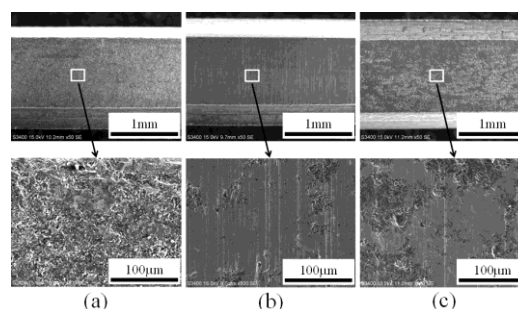
Figure 2 SEM micrograph of piston ring surfaces. (a) New piston ring, (b) lubricated with 15W40 diesel engine oil and, (c) lubricated with nano-oil
