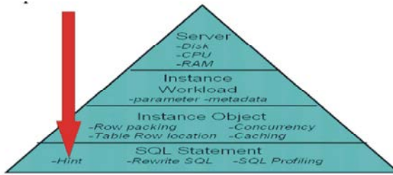
Fig. 3: DBMS tuning hierarchical level [11]
