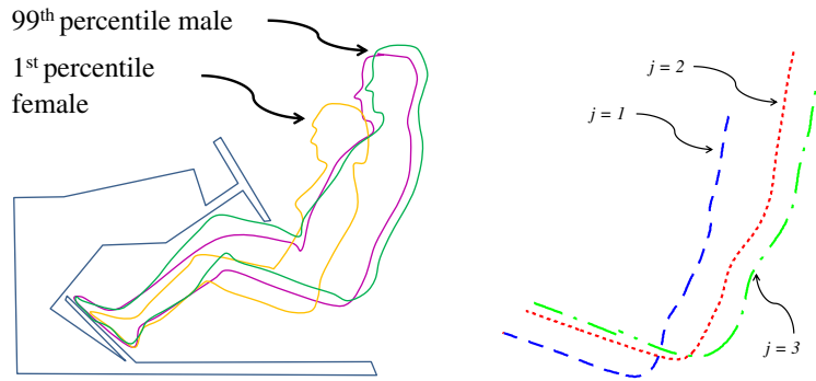
Fig. 12. (a) The silhouettes of a small, an average and a large driver [43]. (b) Seat design profiles that suit the small, average and large drivers from (a).
