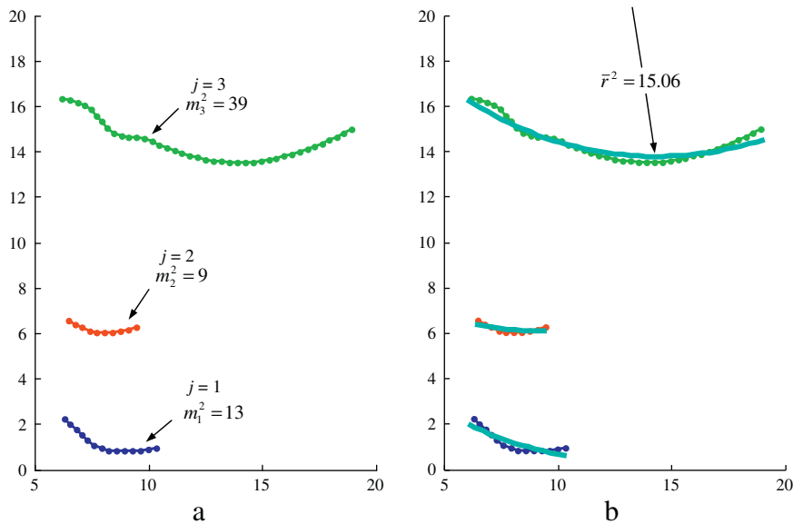
Fig. 7. (a) The second segment from each of three target profiles approximated with a \mathcal{C} -segment. (b) An arc of the same radius, but varying length, approximates the segment on all profiles.
