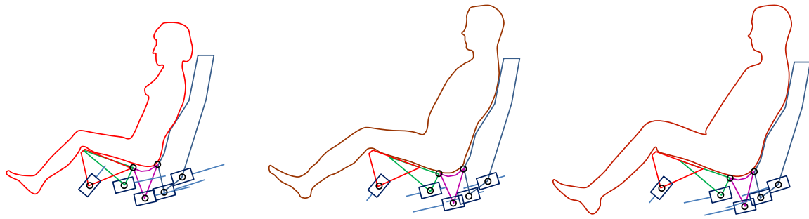
Fig. 14. The results of the mechanization process: (a) The seat is adjusted for a 1st percentile female. (b) The seat accommodating a 50th percentile male. (c) The car seat is positioned for a 99th percentile male.
