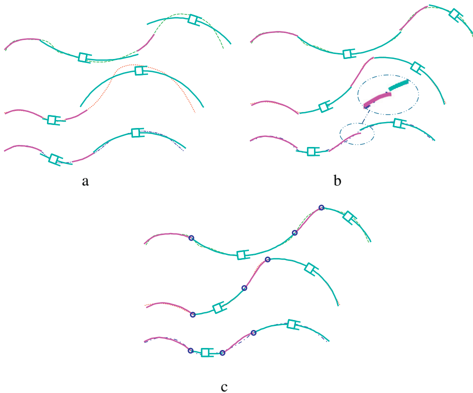
Fig. 8. A rigid-body chain that approximates the target profiles. (a) The chain after the initial segmentation matrix: E_{max} = 1.50 . (b) The chain after the error-reducing iterations: E_{max} = 0.33 . The inset illustrates that segmentation points are not coincident. (c) The joining process unites segmentation points, yet increases the error to E_{max} = 0.34 .
