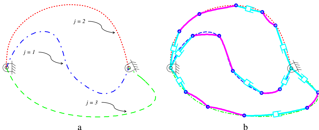
Fig. 11. (a) Fixed-end profiles. (b) The final, rigid-body, shape-approximating chain having E_{max} = 0.18 .
