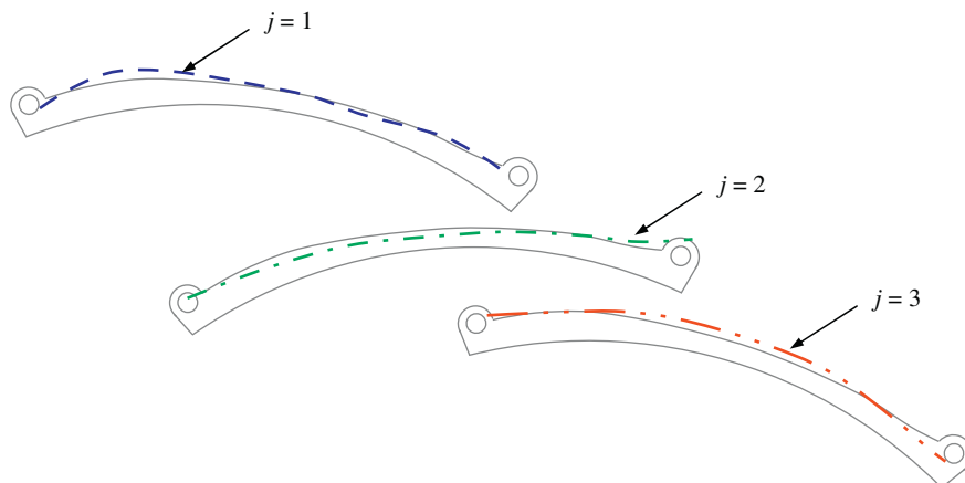
Fig. 4. An \mathcal{M} -segment represents a single revolute-revolute link that corresponds to groups of equal numbered pieces on each target profile.
