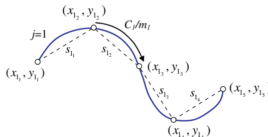
Fig. 2. Design profile (solid) with an approximating target profile (dashed) where points are positioned to give a constant arc length along the design profile.
