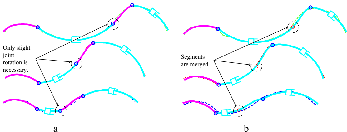
Fig. 10. (a) The original chain consisted of 4 segments resulting in E_{max} = 0.34 , yet one revolute joint exhibited limited motion. (b) The 2nd and 3rd segments were merged into a compound segment, resulting in a three-segment chain with E_{max} = 0.46 .
