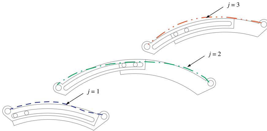
Fig. 5. C-segments are variable arc length groups of pieces consisting of a different number of points on each target profile and represent a revolute–prismatic–revolute chain.
