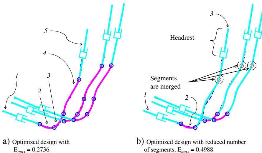
Fig. 13. The three seat profiles can be approximated by the five segment shape-approximating chain in (a). The creation of a compound segment reduces the chain to three segments in (b) with only a modest increase in error.
