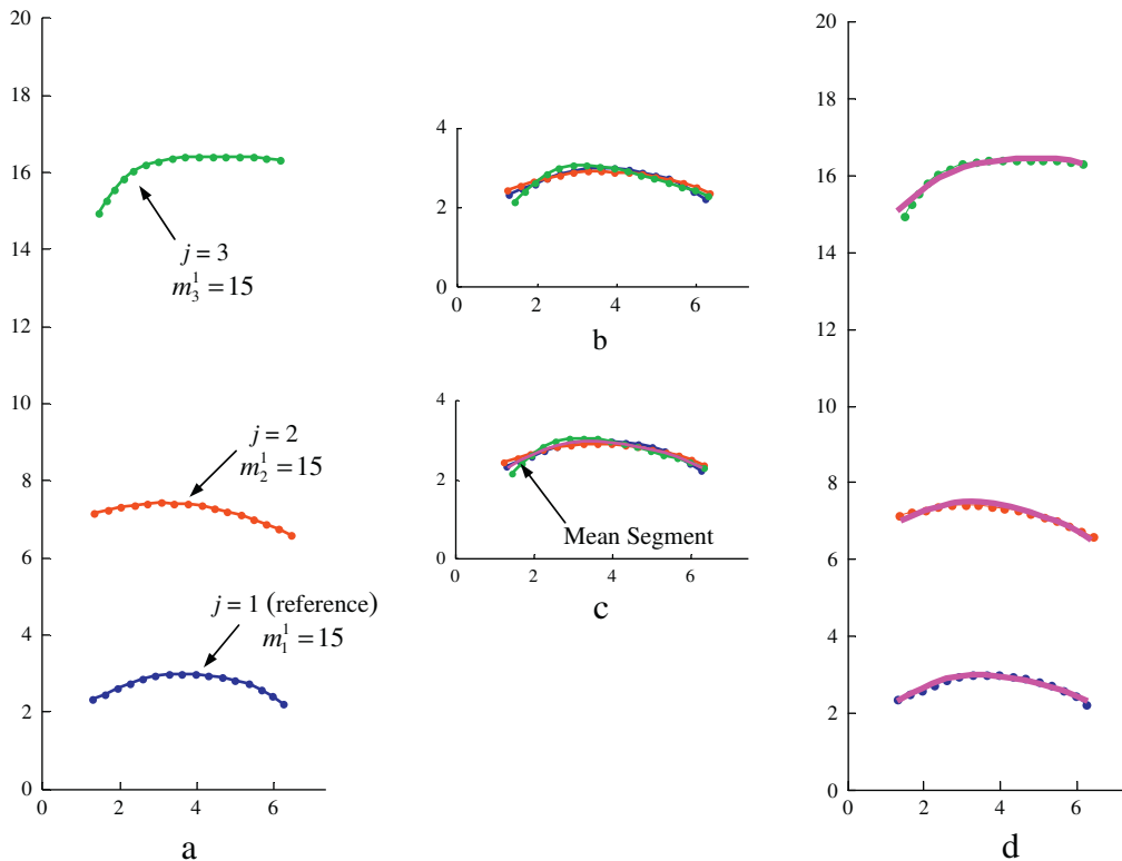
Fig. 6. (a) The first segment from each of three target profiles to be represented by one mean segment. (b) Segments 2 and 3 shifted to reference segment 1 in a distance minimizing transformation. (c) The mean segment generated as the average of the corresponding segment points. (d) The mean segment shifted back to the original segments in another distance minimizing transformation.
