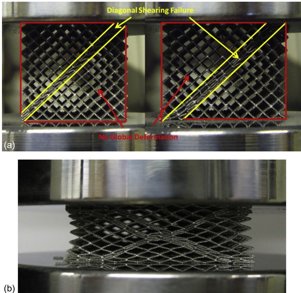
Fig. 6. The quasi-static crush behaviour of (a) 2 repeat tests for the SLM Ti64 lattice block and (b) HIPed Ti64 lattice block (Manufacturing parameters: Power = 180 W and Exposure Time = 500 \mu s).
