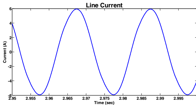
Fig. 10: Line current
