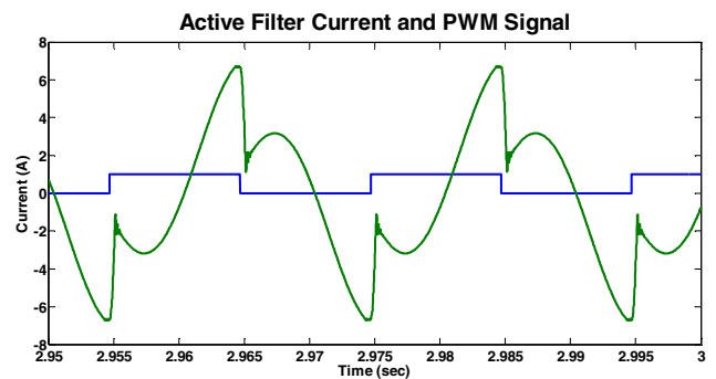
Fig. 7: Active filter current and PWM signal
