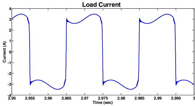
Fig. 8: Load current
