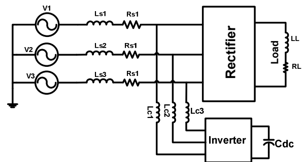
Fig. 1: Three phase active filter
