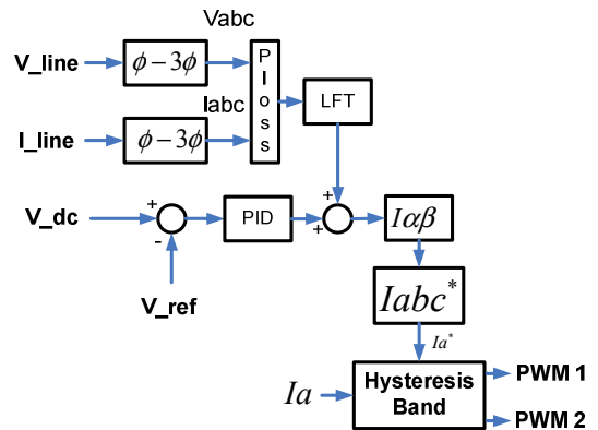
Fig. 3: Control strategy
