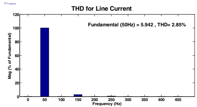
Fig. 13: THD for line current
