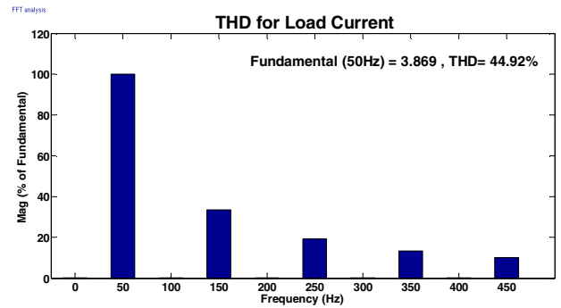
Fig. 12: THD for load current
