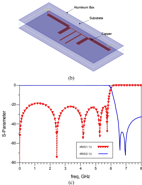
Fig. 4 : (a) Layout of generalized Chebyshev lowpass filter (b) 3-D view of Generalize Chebyshev lowpass filter (c) Simulated frequency response of the generalized Chebyshev lowpass filter in suspended stripline structure
