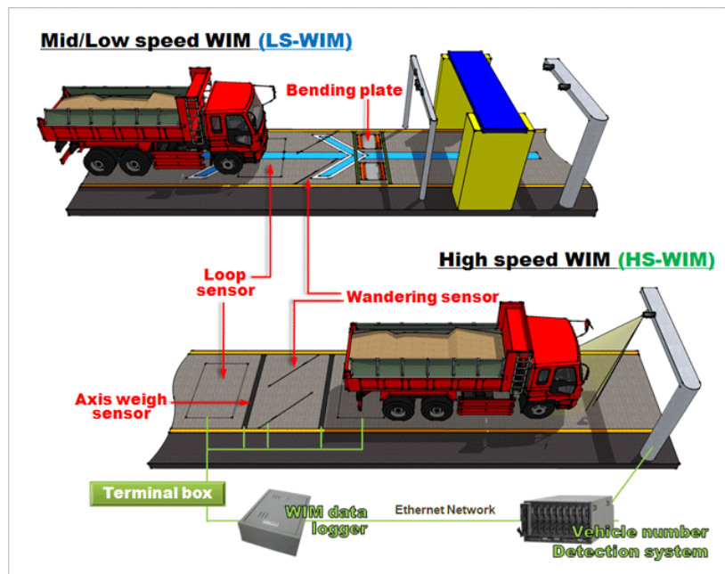
Figure 5: Weight-in-motion Sensor.
