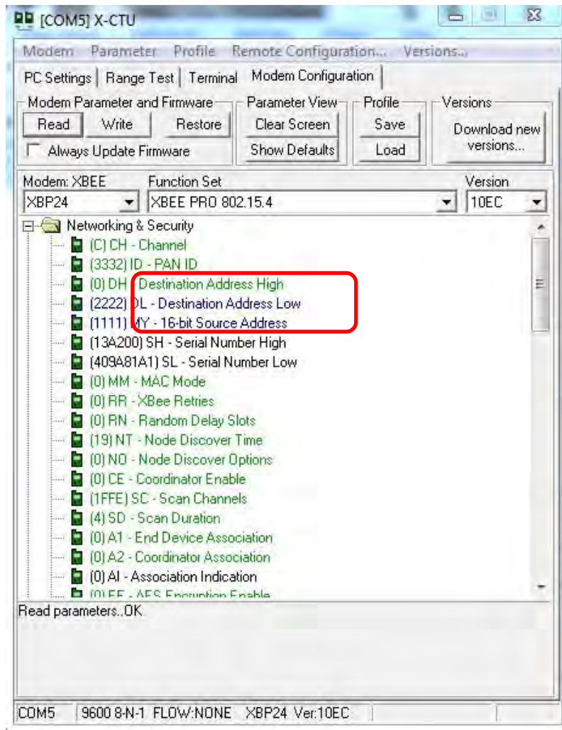
Figure 16: Modem Configuration
