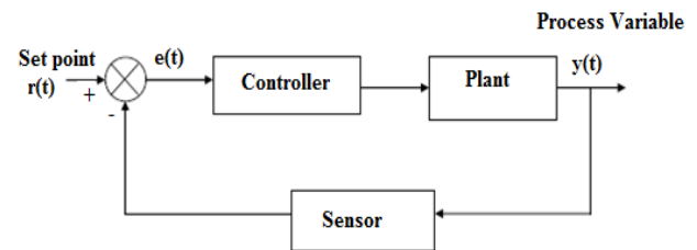
Figure 1: Control System
