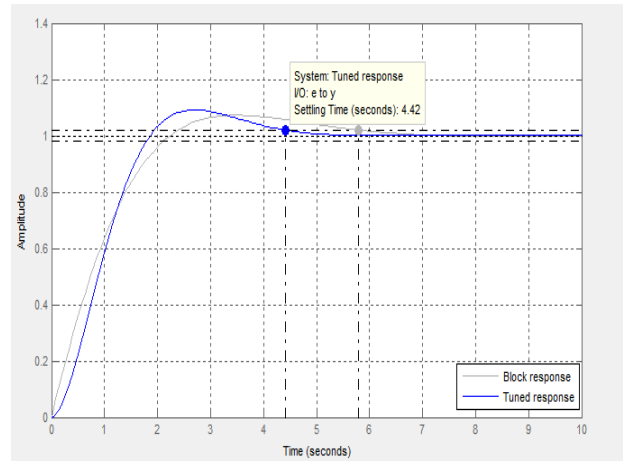
Figure 9: PID Controller Settling Time (Ts)
