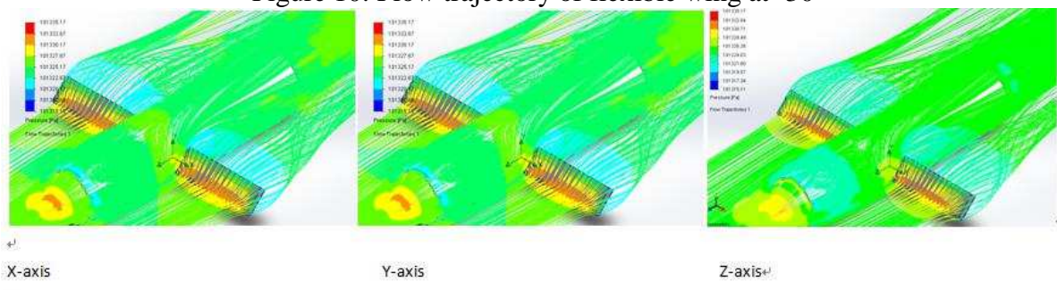
Figure 11: Flow trajectory of flexible wing at -45°
