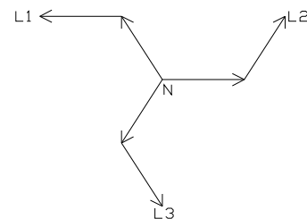
Figure.3: Wye-Zigzag Transformer Phasor Diagram
