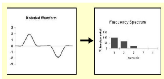
Figure. 1 Relationship of Distorted Waveform with Frequency Spectrum
