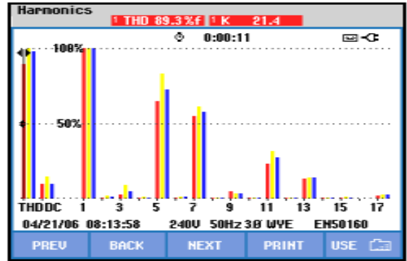
Balanced Load
