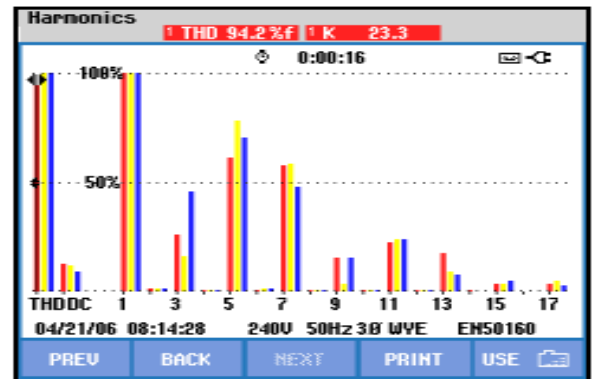
Unbalanced Load
