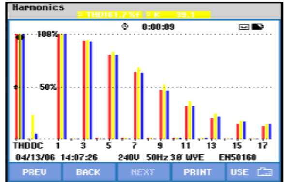
Fig.5b: Spectrum representation of harmonics for direct contact configuration (no transformer connection)
