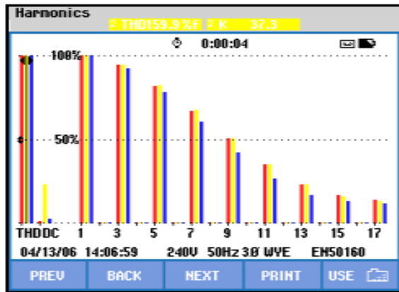
Fig.5a: Spectrum representation of harmonics for direct contact configuration (no transformer connection) Balanced Load
