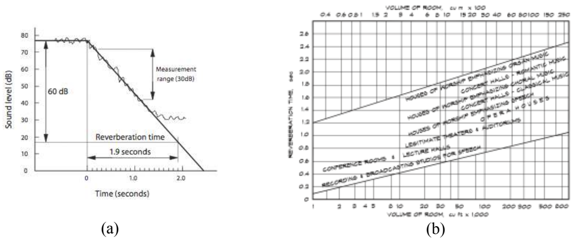
Figure 1:(a). Reverberation time [6] and (b) recommended reverberation time according to room volume and functions [5].
