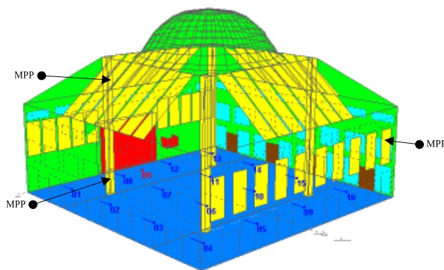
(a) (b) Figure 6: (a) CATT model of strips of MPP installed in a mosque and (b) simulated reverberation time.
