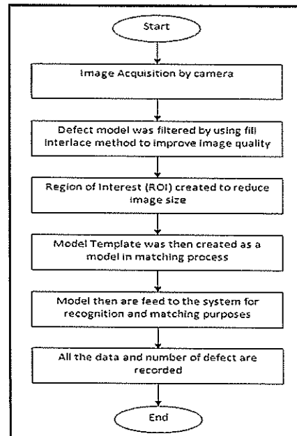
Figure 1: Suggested vision algorithm
