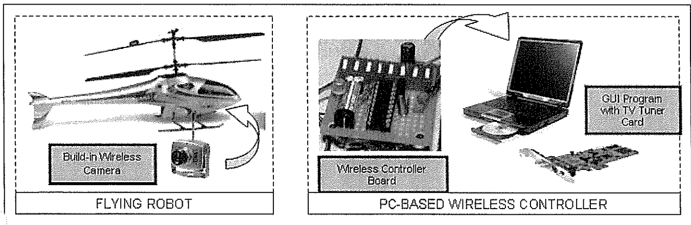
Figure 2: The Overall Block Diagram of PC Based Wireless Controller for Flying Robot
