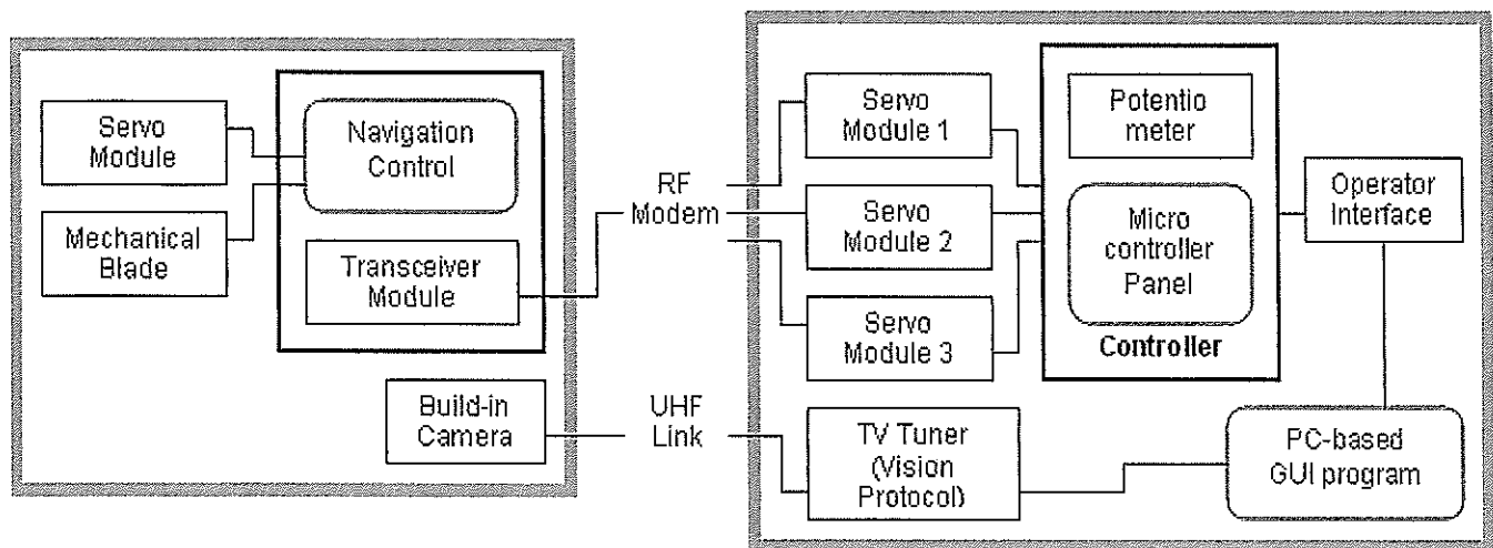
Figure 3: System Functional Block Diagram of the Project Development
