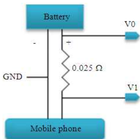
Fig. 1. Block diagram for the hardware component
