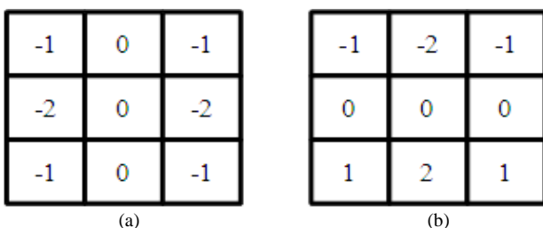
Fig. 4. (a) The vertical direction Sobel 3×3 mask. (b) The horizontal direction Sobel 3×3 mask
