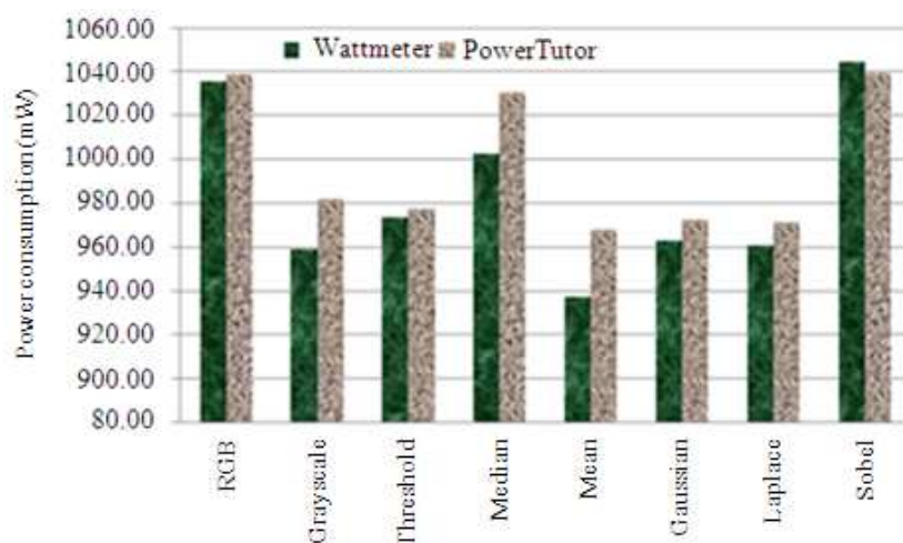
Fig. 6. The mean of 30 average power consumption in one second obtained from wattmeter and PowerTutor application for the eight image processing methods
