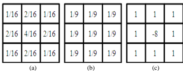
Fig 3. (a) Gaussian mask, (b) Mean filter mask, (c) Laplacian mask
