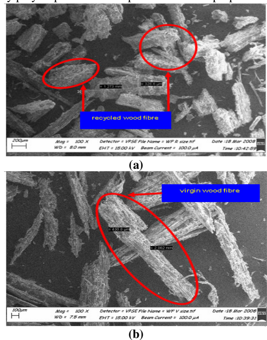
Fig. 9. SEM micrograph showing (a) recycled wood fibre, and (b) non-recycled wood fibre
