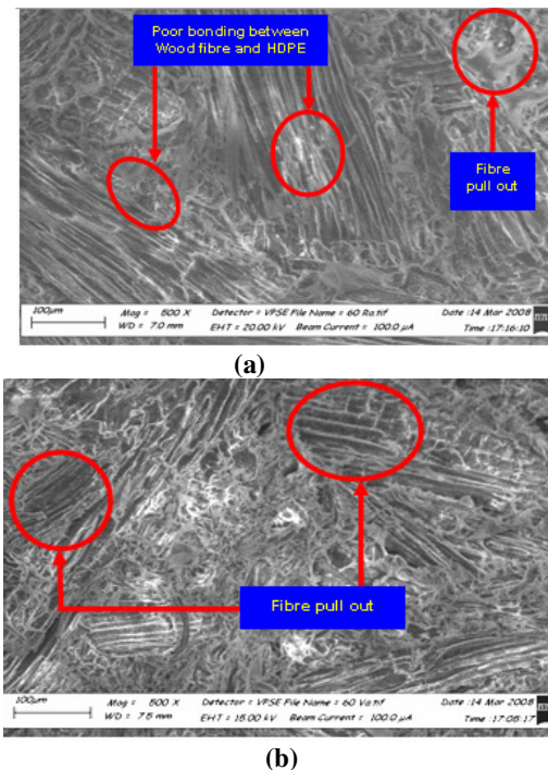
Fig. 7. Fracture surface of tensile specimen for 40% filler in (a) recycled WPC, and (b) non-recycled WPC
