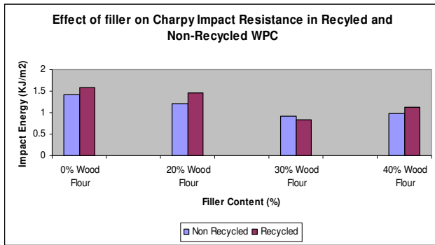
Fig. 5. Impact Energy ( \text{KJ/m}^2 ) of the Recycled and Non-Recycled WPC
