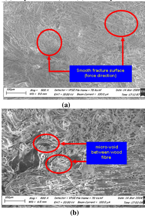
Fig. 8. Fracture surface of tensile specimen for 30% filler in (a) recycled WPC, and (b) non-recycled WPC
