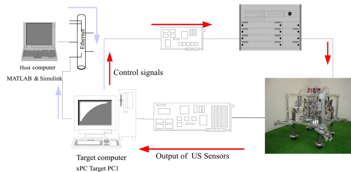
Fig. 3 Experimental setup
