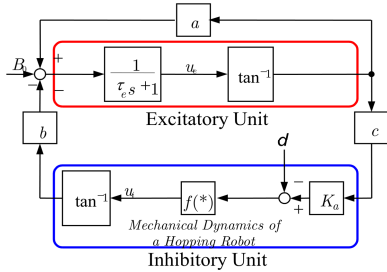
Fig. 4 CPG model
