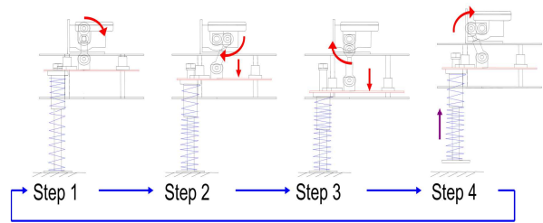
Fig. 2 Hopping mechanism
