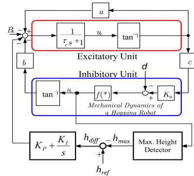
Fig. 5 Reference height control system
