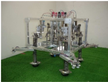
Fig. 1 Quadruped hopping robot
