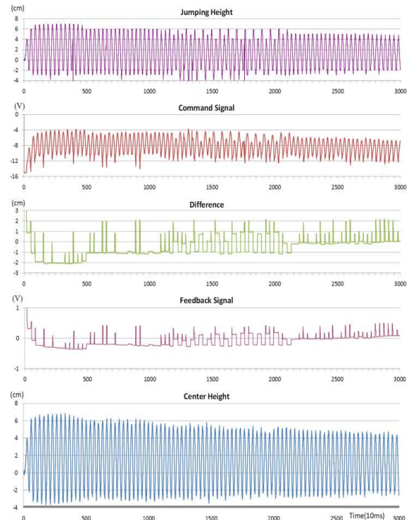
Fig. 8 Experimental result by using PI controller
