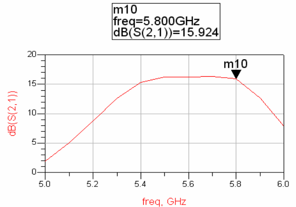
Figure 4: Forward Gain
