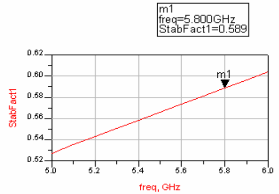
Figure 2: LNA stability
