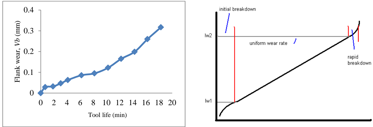
Figure 2 Flank wear-tool life graph (a) Experiment 1: v = 60 \text{ m/min} , f = 0.2 \text{ mm/revolution} , d = 0.3 \text{ mm} ; (b) Typical wear rate (G.K. Lal, 2005)
