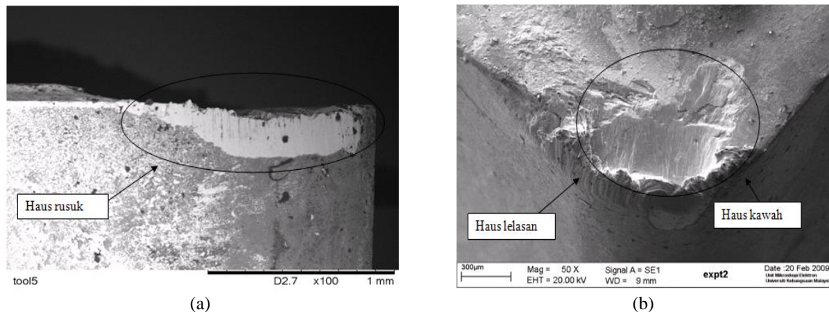
Figure 5 Severe flank wear (a) abrasive wear and notch wear (b)
