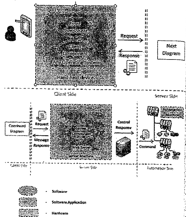
Fig. 1 System Architecture
