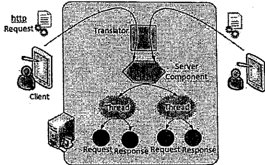
Fig. 2 Multithreading
