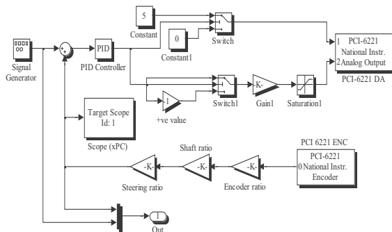
Figure 5. Position tracking controller developed for HILS
