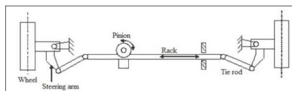
Figure 1. The rack and pinion steering linkage system
