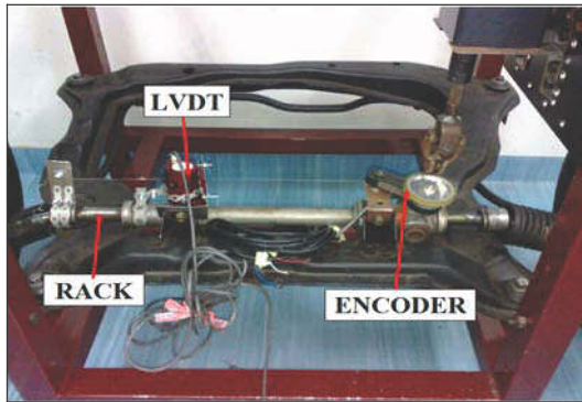
Figure 4. HILS set up for rack and pinion steering linkage
