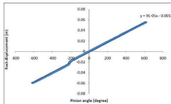
Figure 7. Graph of rack displacement versus pinion angle
