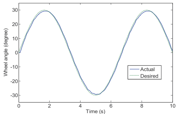
Figure 6. Positioning tracking for DC motor
