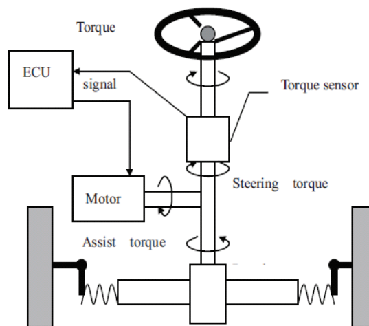
Figure 1. Electric power steering (EPS) schematic (photo reprinted from [18])
