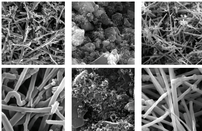
FIGURE 1 SEM images at 2 micron and 500nm scale for NC300 (a, d), NC200 (b, e), and Commercial CNT (c, f)
