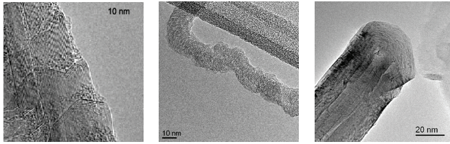
FIGURE 2 TEM images for a) NC300, b) NC200, and c) Commercial CNT
