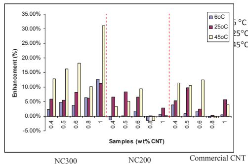
FIGURE 4 Percentage enhancement of nanofluid based nanocarbon
